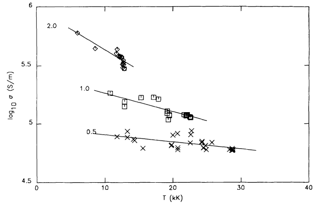
FIG. 9. Measured conductivity versus temperature for densities of 2.0, 1.0, 0.5 \text{g}/\text{cm}^3 . Solid lines are linear least squares fits to the data.
